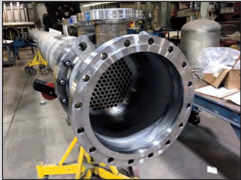
Fabricated Equipment
